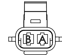
MATING VIEW OF 15300008 CONNECTOR A=GROUND TABS B=CENTER CONTACT
