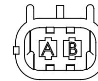
MATING VIEW OF 15300002 CONNECTOR A=BLACK (GROUND) B=RED (12V DC)
